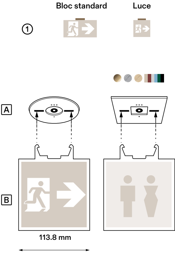
Luce EP4, recessed ceiling-mounted, brass with Meljac finish.
